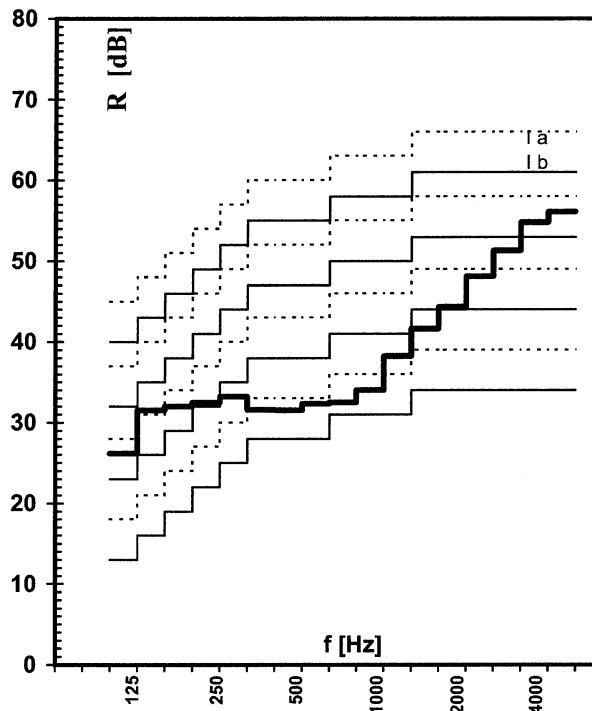
INTERIOR WALLS - BINNENWANDEN - CLOISONS
