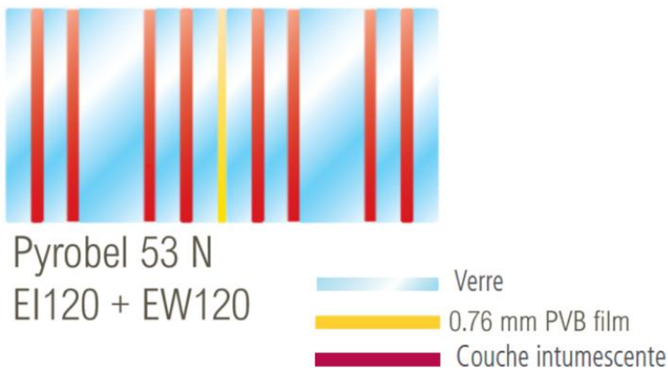
Figure 1: Structure of a Pyrobel 53N Low-Carbon Stock-Size
