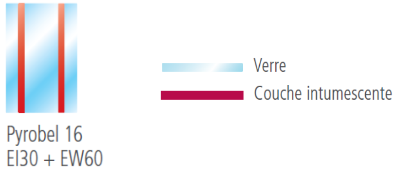
Figure 1: Structure of a Pyrobel 16 Low-Carbon Stock-size
