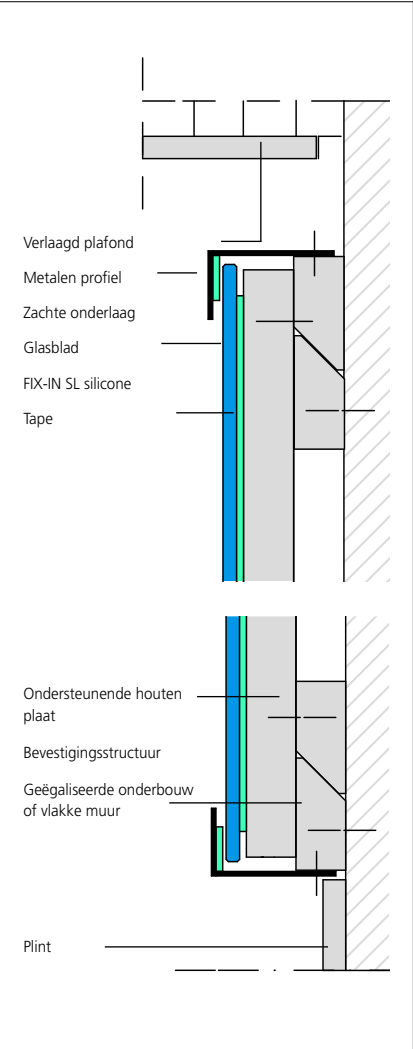
VERTICALE dwarsdoorsnede
