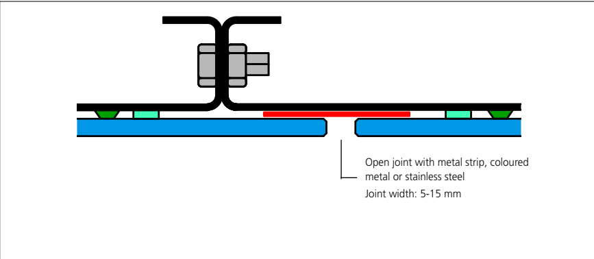
ELEVATOR CAR: HORIZONTAL CROSS SECTION WITH COLOURED JOINT
