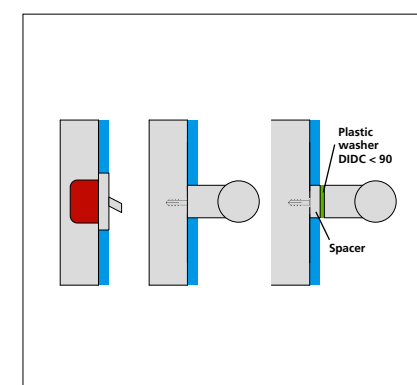
RIGHT: NO PRESSURE EXERTED ON THE ANNEALED GLASS
