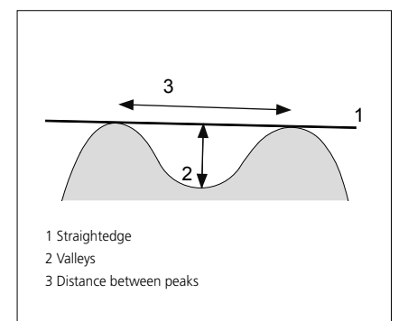
MEASUREMENTS OF FLATNESS
