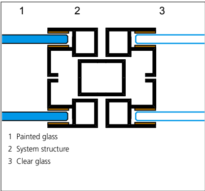
METAL STRUCTURE: HORIZONTAL CROSS SECTION
