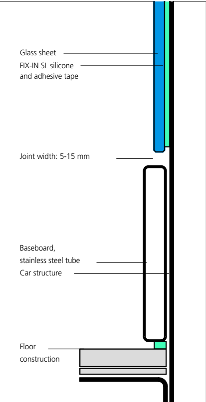
ELEVATOR CAR: VERTICAL CROSS SECTION WITH BASEBOARD
