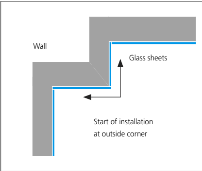
SEQUENCE OF MOUNTING: FLOOR PLAN
