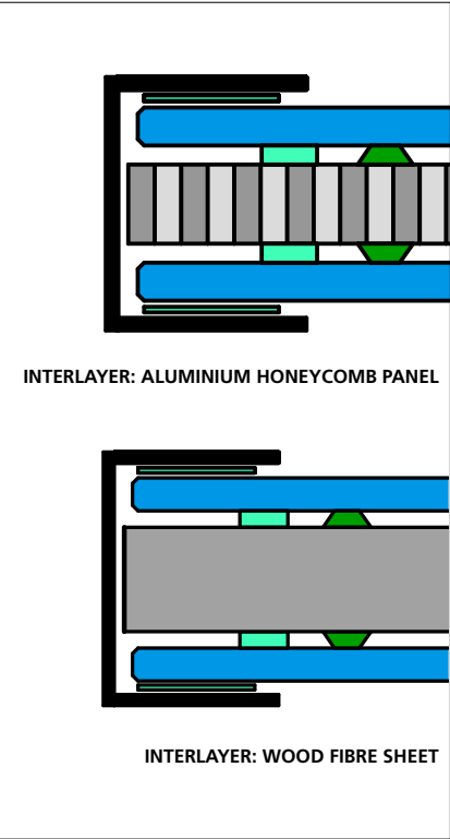
DOOR STRUCTURES
