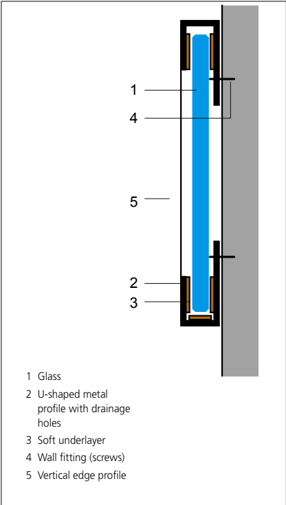
MECHANICAL FITTING: MIROX
