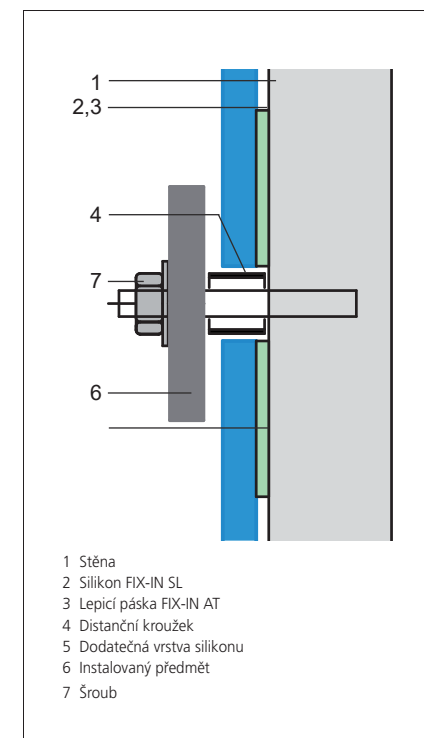
INSTALLATION USING SLEEVES
