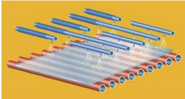
Fig. [2]: Hot air distribution on the upper side of the glass
