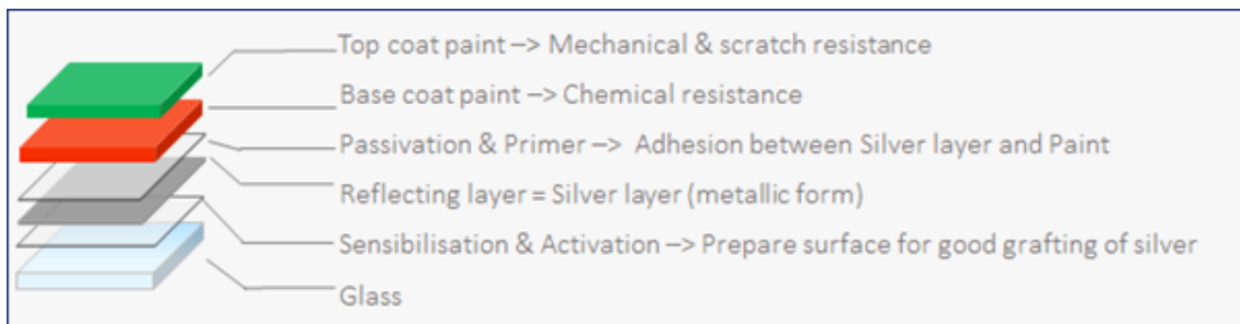
Figure 1 : Matelac Silver composition
